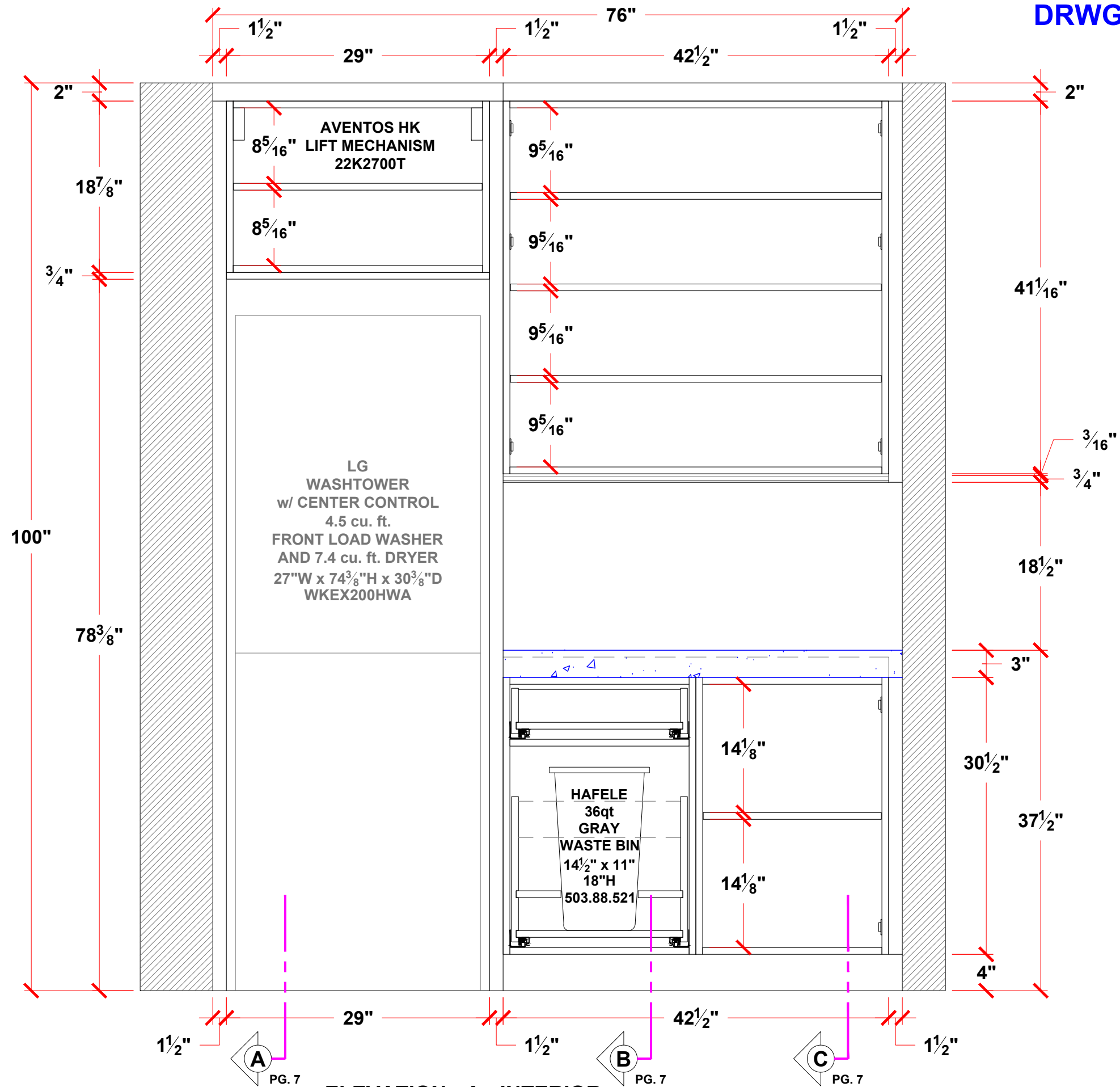
ELEVATION - A - INTERIOR GLIKIN - LAUNDRY (02162C-07)
