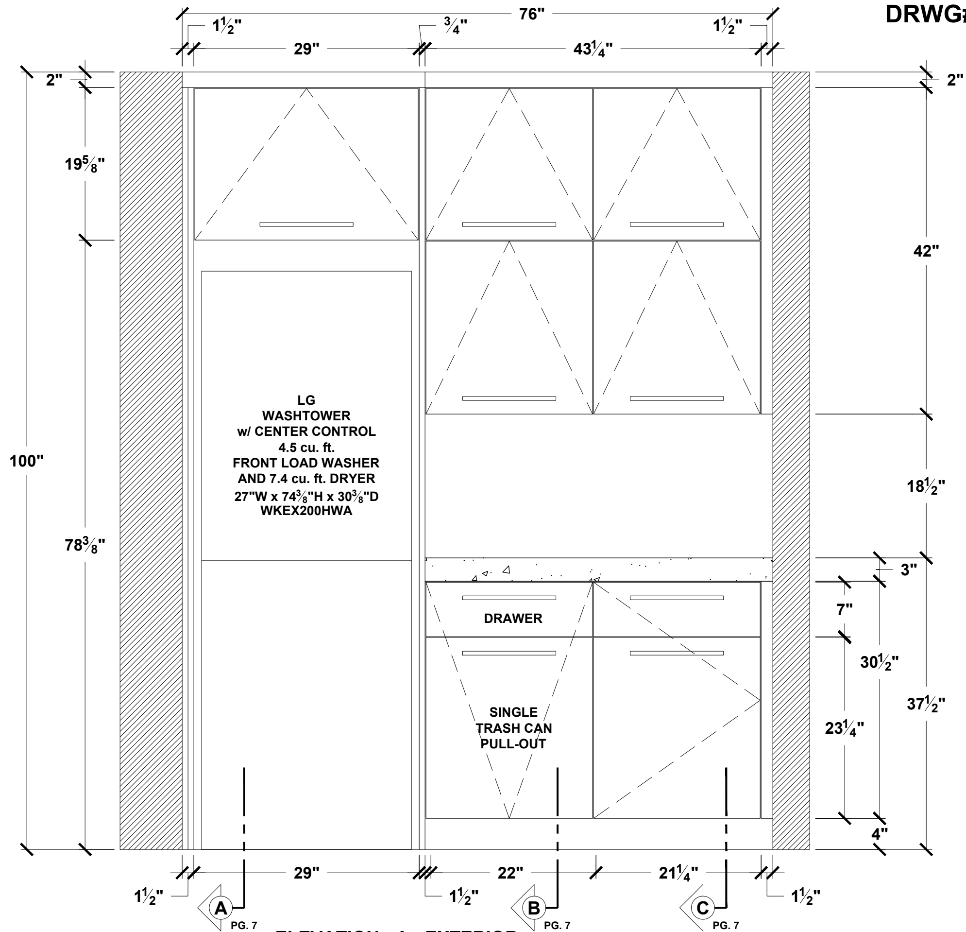
ELEVATION - A - EXTERIOR GLIKIN - LAUNDRY (02162C-07)
