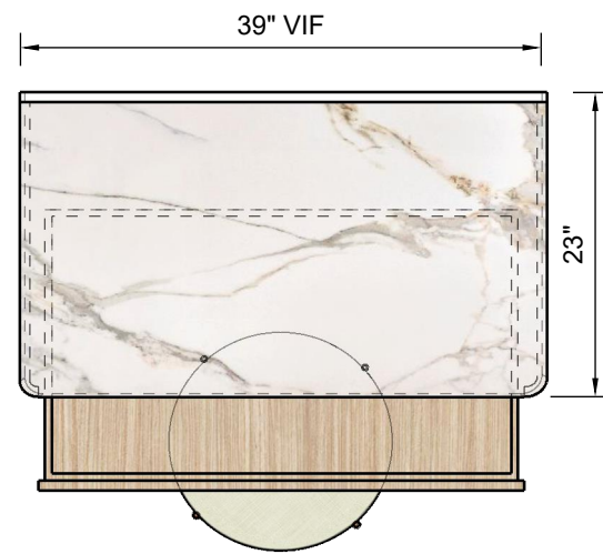
TOP VIEW Scale 1:16
