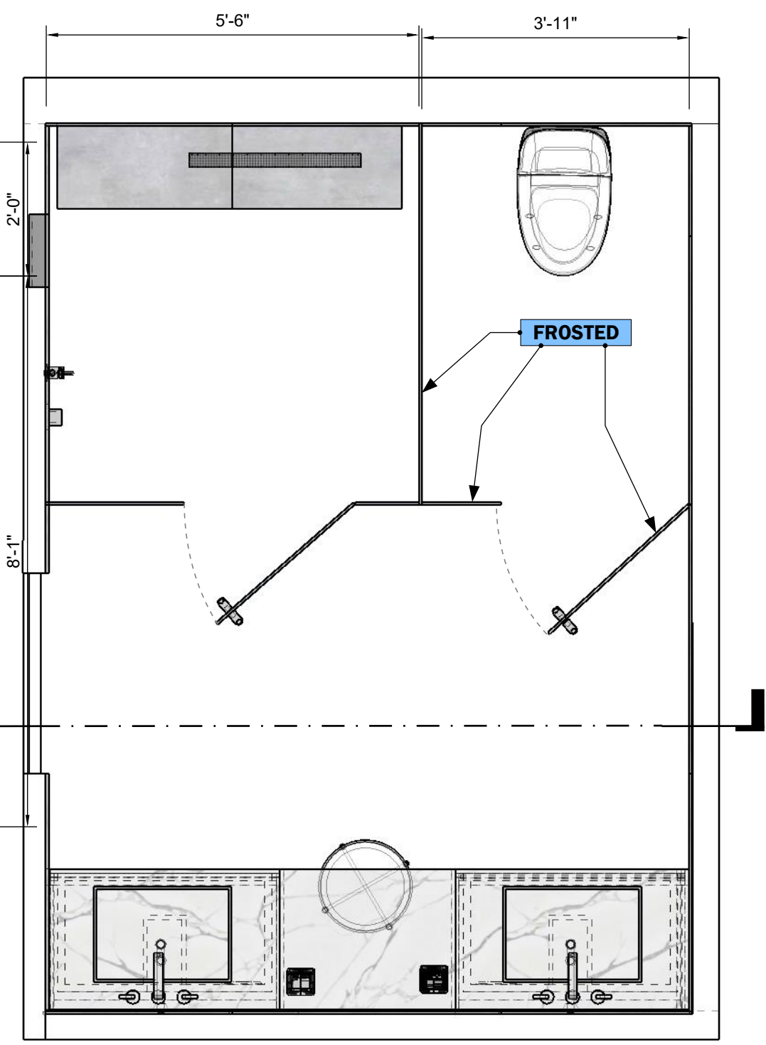
TOP VIEW Scale 1:24
